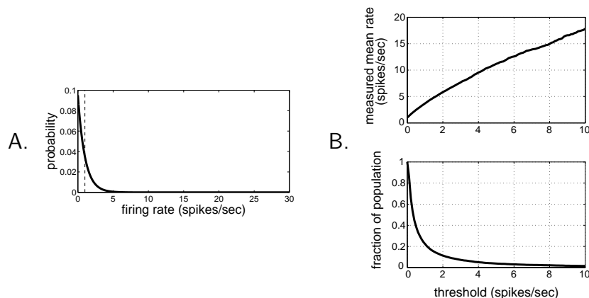
Figure 2: Sampling bias. A. Exponential firing rate distribution with a mean of 1 Hz (dashed line denotes mean). B. Resulting overall mean-rate of the population (top), and fraction of the population captured (bottom), as a result of recording from neurons only above a given mean firing-rate (threshold).
